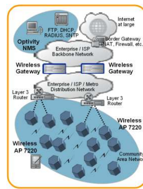
Figure 3 – The Wireless Mesh Network
